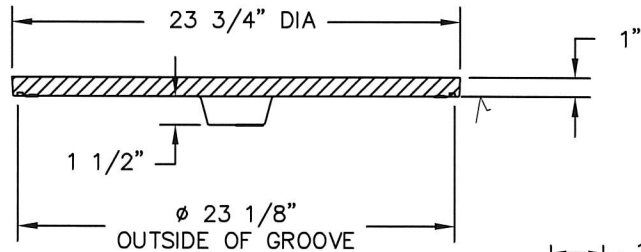
COVER SECTION
