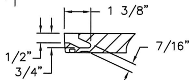
PICKHOLE DETAIL
